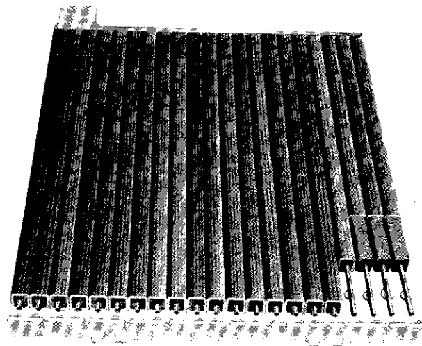
Tubular plate construction
