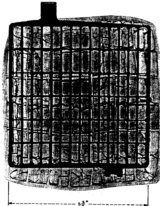
Corroded positive lead calcium plate with original grid overlaid to indicate initial dimensions.
